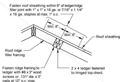
Figure 27. Ridge Filler Option for Hinged Roof
