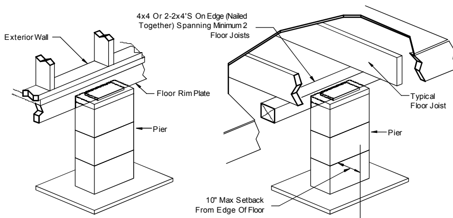
Figure 15. Perimeter supports
