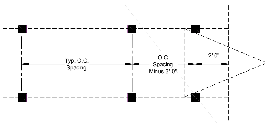
Figure 10. End of beam piling exception
